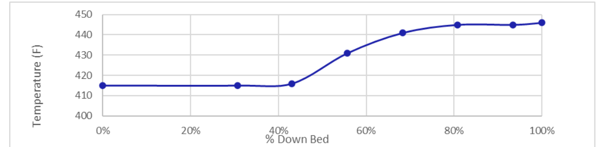
KATALCO 83-3 temperature profile after 3 years on-line
